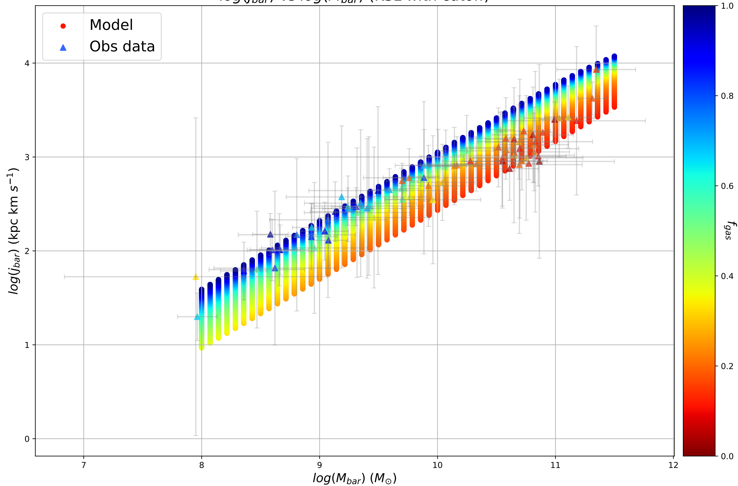
\log(j_{\text{bar}}) vs \log(M_{\text{bar}}) (KSL with cutoff)
